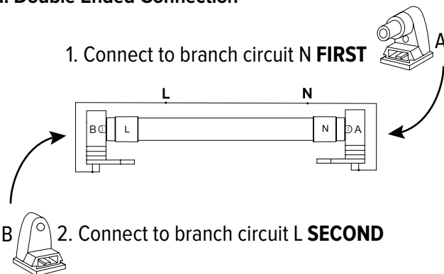
Fig 1. Double Ended Connection
