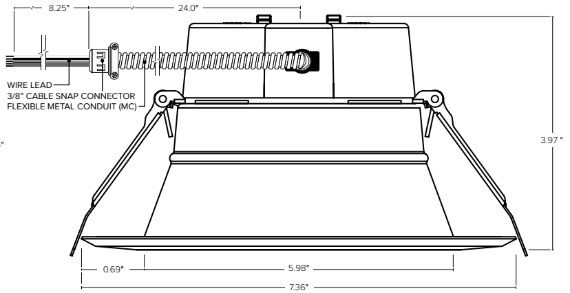
6" Fixture
