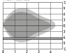
Wall mounted
